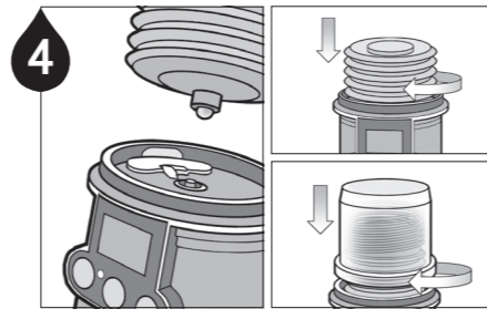
4 Purge the grease pouch until grease comes out of the tip. Carefully screw the grease pouch in by turning clockwise. Do not over tighten. Refit the top housing on the unit and turn clockwise until it clicks.
