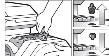
5 Remove the grease nipple and install appropriate adaptors.
